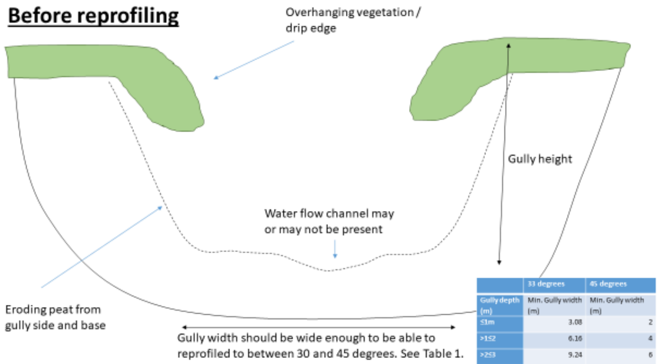
Figure 19 Diagram of a gully before reprofiling
