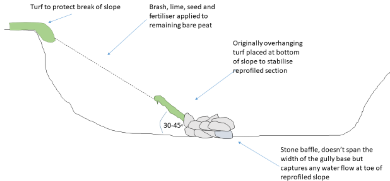
Figure 23 After reprofiling - stone baffle
