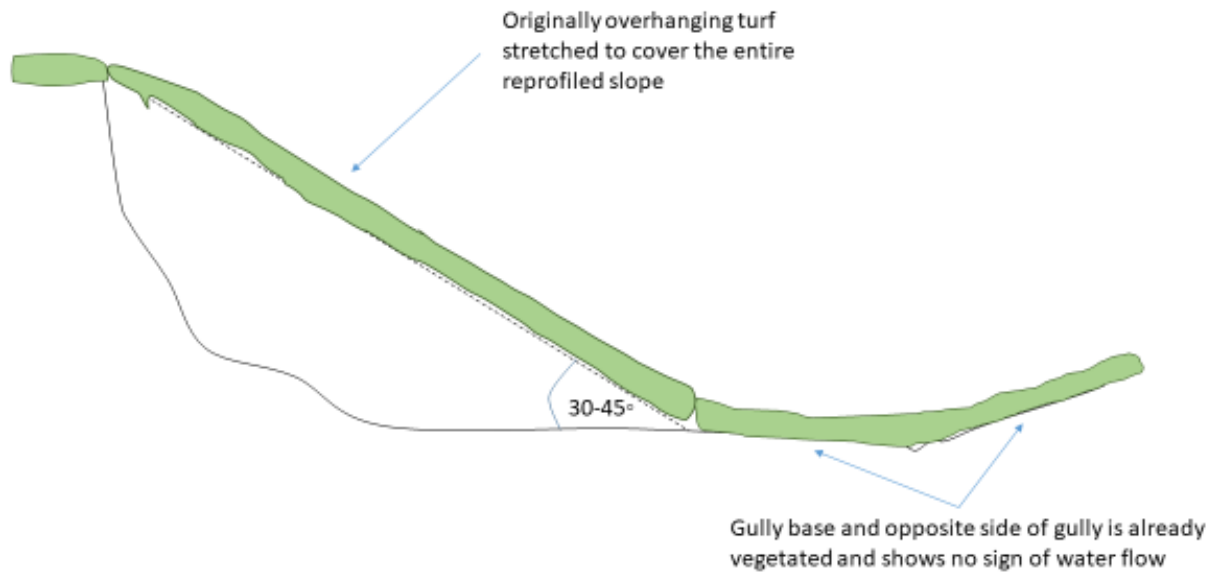
Figure 20 After reprofiling - turf stretched across the entire slope
