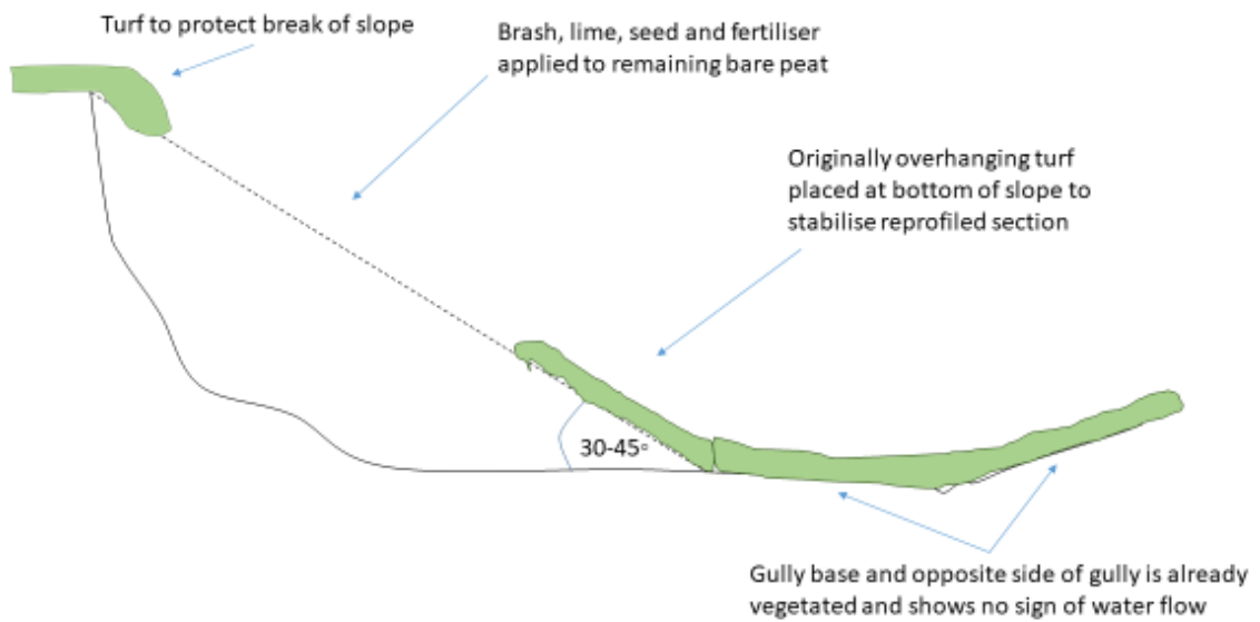
Figure 21 After reprofiling - not enough turf to stretch across entire slope
